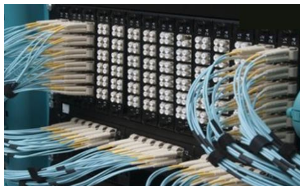
FAS-NET MPO Chassis, 14 Vertical Slots, 3U
